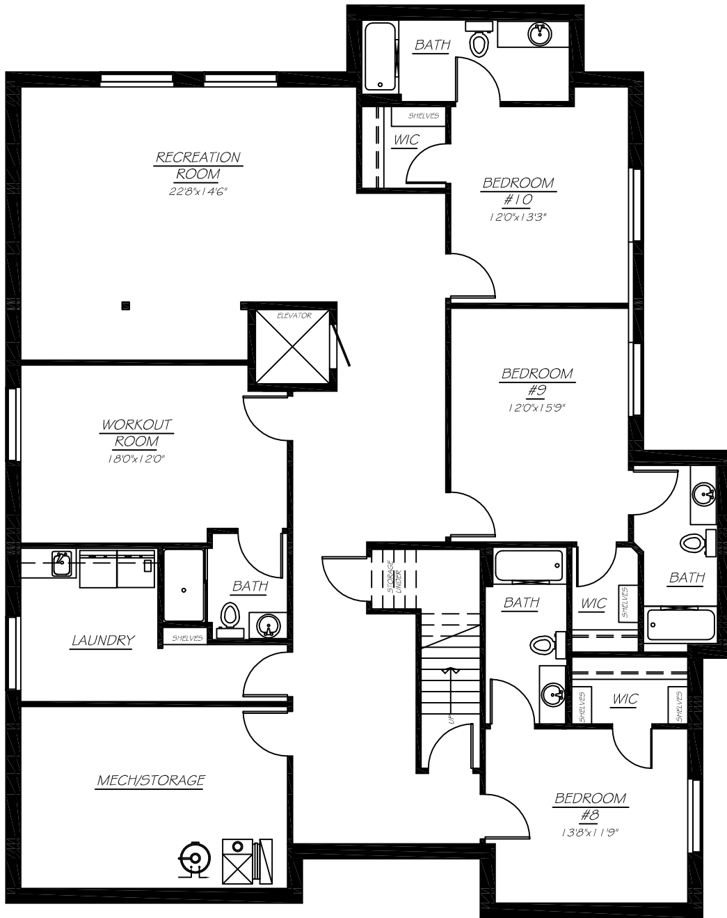
LOWER LEVEL
